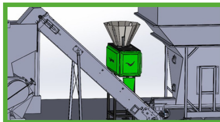
The unit is placed directly next to the conveyor belt that transports the material from the material container to the pellet mill
