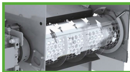
Exchangeable, screwed sieve with different sieve diameters. Discharge via suction, discharge screw or conveyor belt
